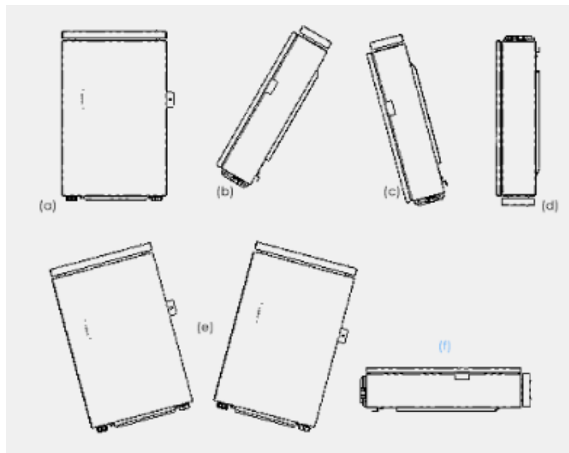
Figure 10 - Mounting Orientation
