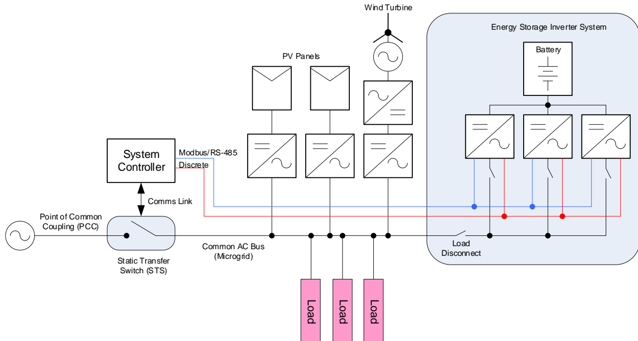
Figure 32 - Island Mode Capable System Block Diagram
