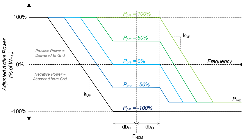
Figure 24 - Frequency/Watt Configuration
