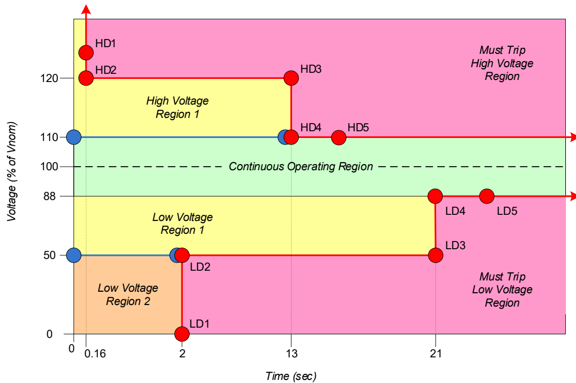
Figure 28 - Voltage Ride Through IEEE 1547-2018 Configuration
