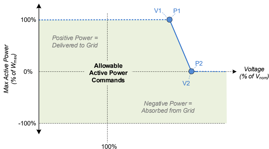
Figure 23 - Volt/Watt Configuration
