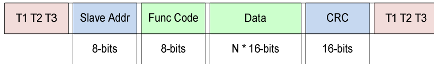
Figure 32 - RTU Message Frame (PDU) Format
